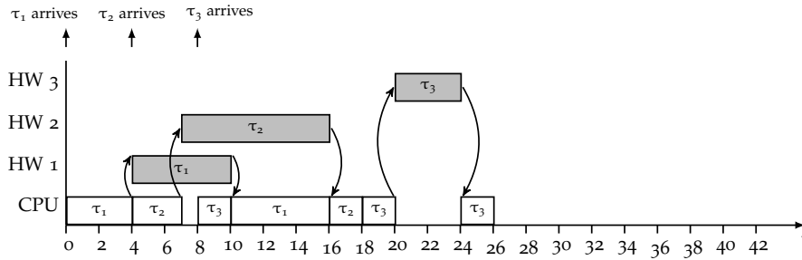
(a) Using FPGA in parallel (suspension aware).
