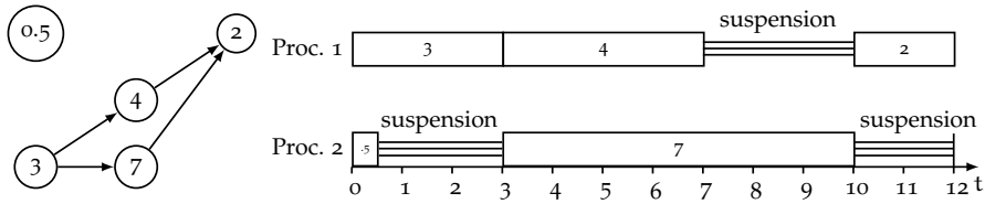
Figure 3: An example of partitioned DAG schedule.
