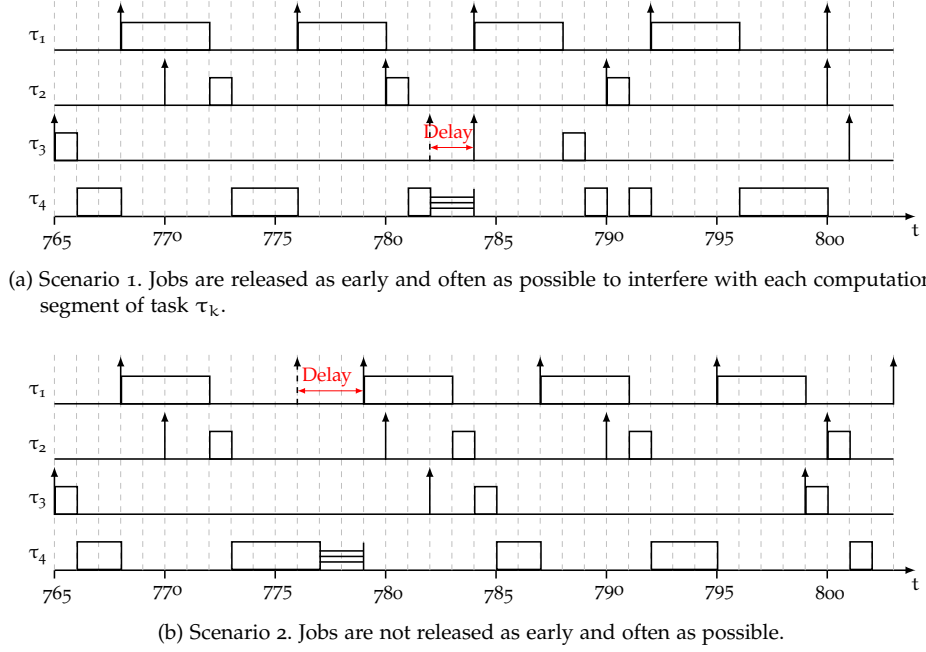
Figure 7: An example based on the task set in Table 8 showing that releasing higher-priority jobs as early and often as possible to interfere with each computation segment of task \tau_k may not always cause the maximum interference on a self-suspending task.
