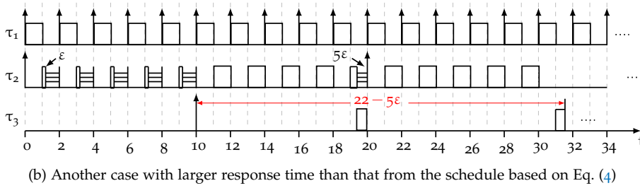
Figure 4: A counterexample for the response time analysis based on Eq. (4) by using the task set in Table 5.
