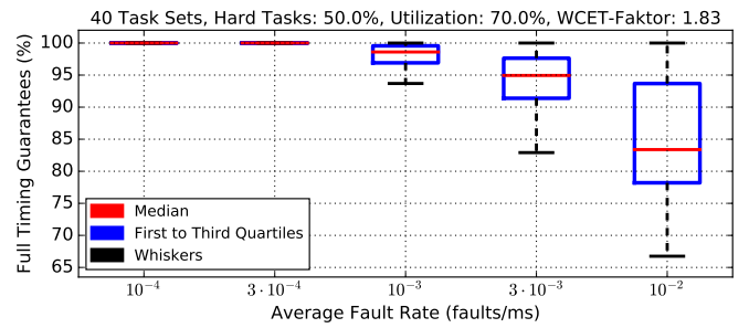
Fig. 5: Percentage of Time with Full Timing Guarantees for task sets with critical utilization under different fault rates.
