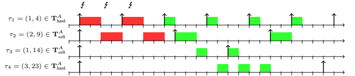
Fig. 6: Faults will not necessarily lead to deadline misses. Tasks characterization: (C_i^N, T_i) , with C_i^A = 2 \cdot C_i^N and D_i = T_i . Three occurring faults ( \zeta ) lead to prolonged execution for the red colored jobs of \tau_1 and \tau_2 due to error recovery. However, \tau_4 still meets its deadline.
