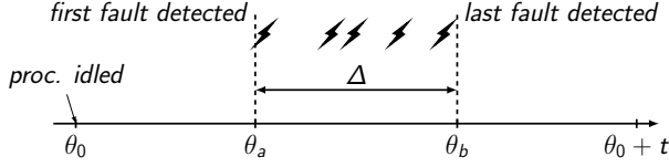
Fig. 2: The illustration of an busy interval of length t undergoing an interval of burst fault [\theta_a, \theta_b] equal to length \Delta .
