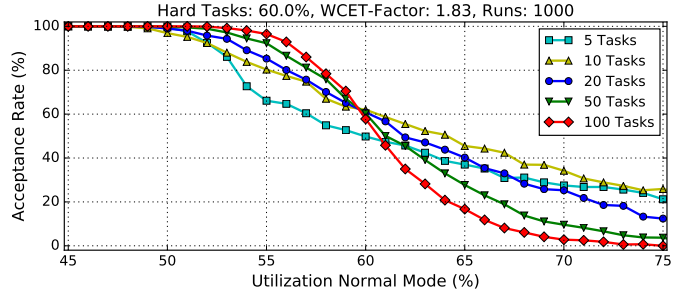
Fig. 8: Acceptance Rate for Different Set Sizes.
