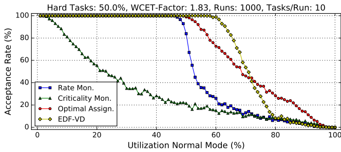
Fig. 3: Acceptance rate for 10 tasks/run.
