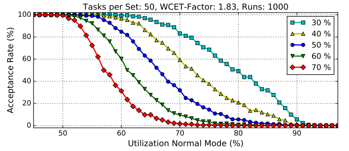
Fig. 7: Acceptance Rate for Percentages of timing strict tasks. The acceptance rate drops earlier if the percentage of hard tasks is higher.
