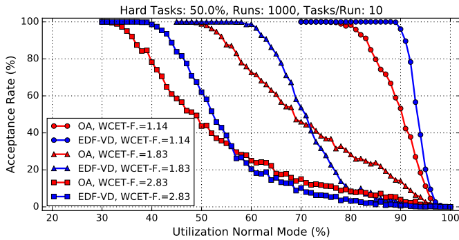
Fig. 4: Comparison of Optimal Assignment and EDF-VD.
